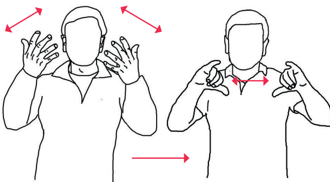
Weather Chart
