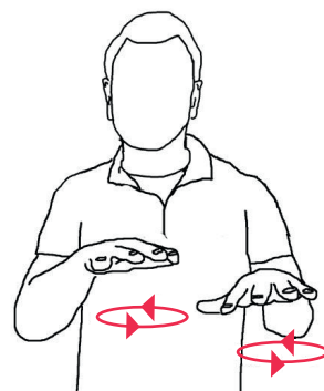
Variable (VRB)
